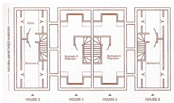
Copse Mews - Second Floor
